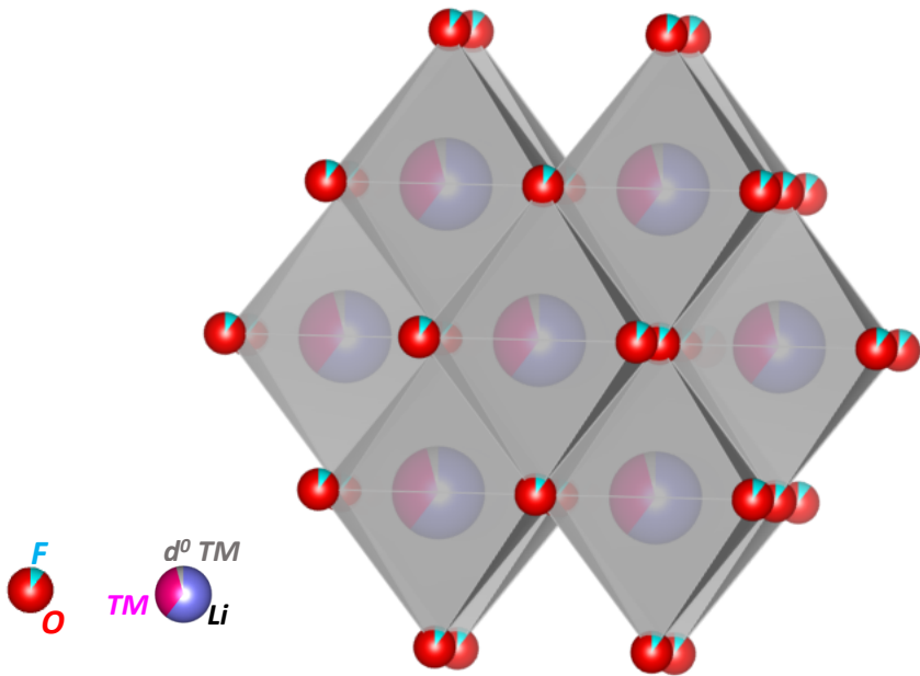
Cation-Disordered Rocksalt Oxyfluoride Cathode (DRX)
