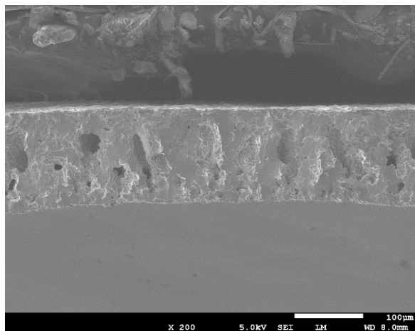
Phase inversion
