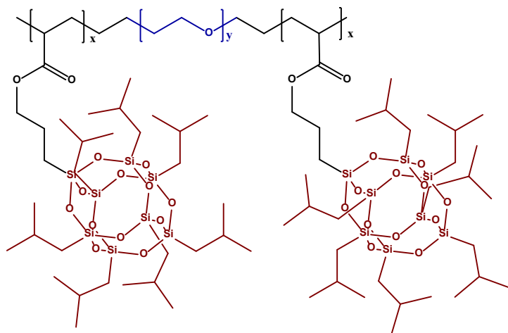
Triblock copolymer
