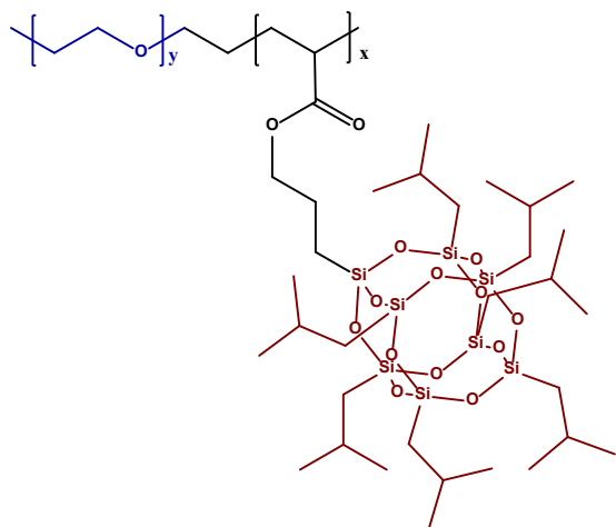
Diblock copolymer
